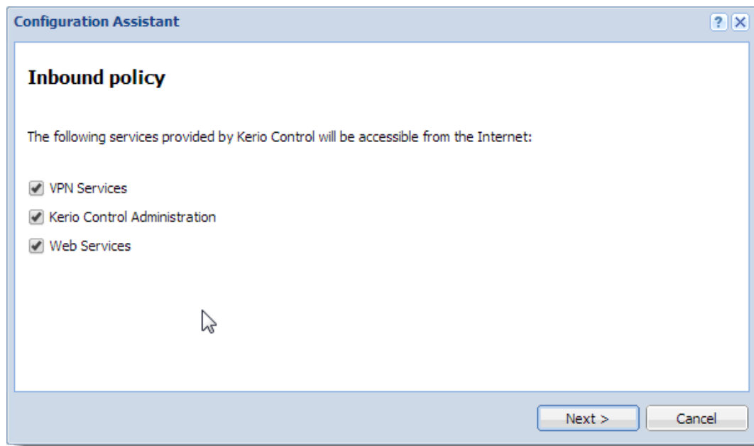
Figure 2 Inbound policy
